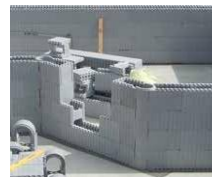
The use of hinge elements to shape corners at any angle.
