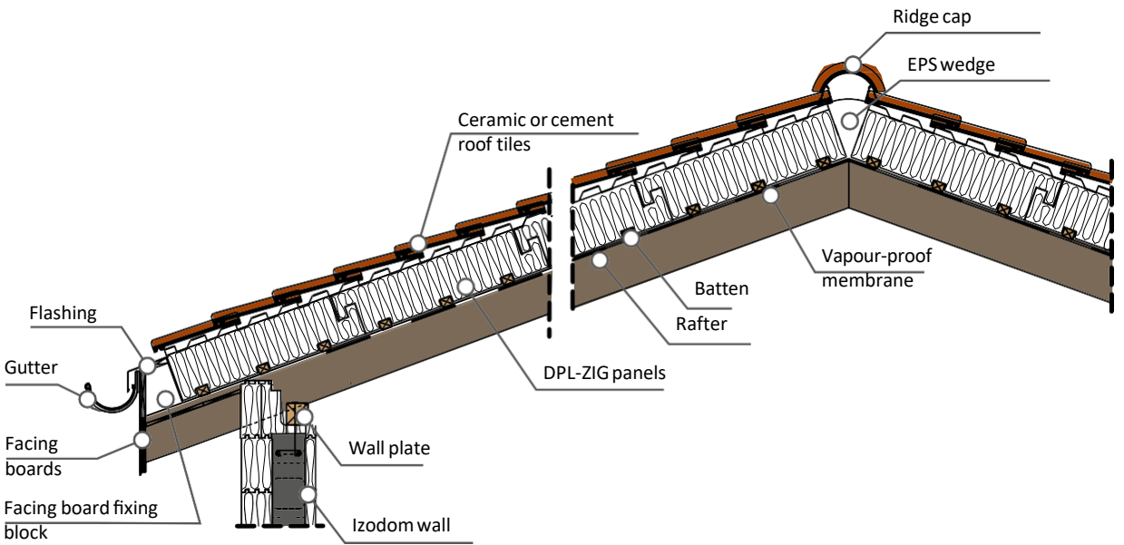
Fig. C. View illustrating a variant of roof plain tiling.
