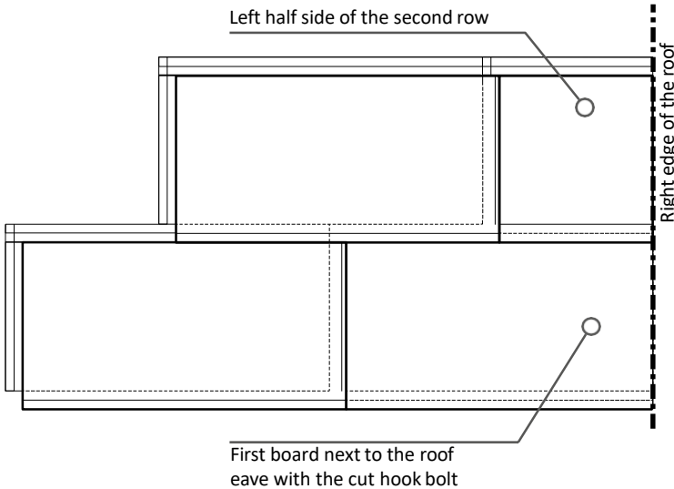
Fig. a Schematic placement of the roof slab.
